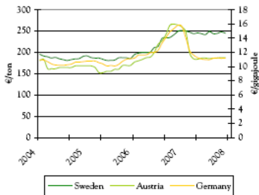
Wood-pellet prices in Europe, 2004-2008
